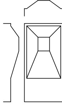
TYPE M Safety ledge upgrade to hopper shape
